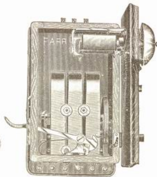
No. 2 Bridging Magneto Bell
