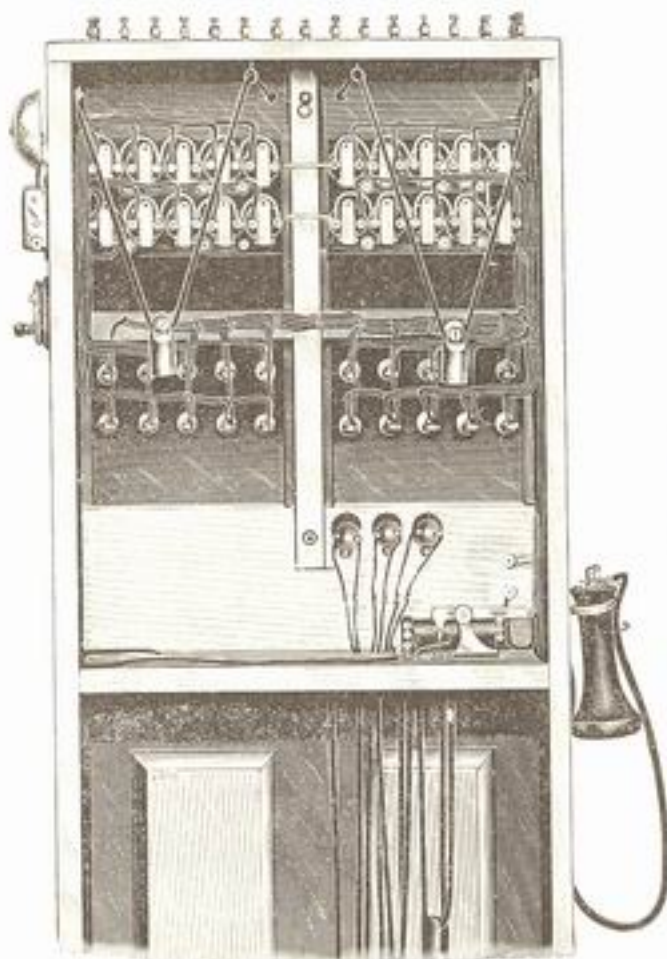
No. 1 SWITCH BOARD Back View.
