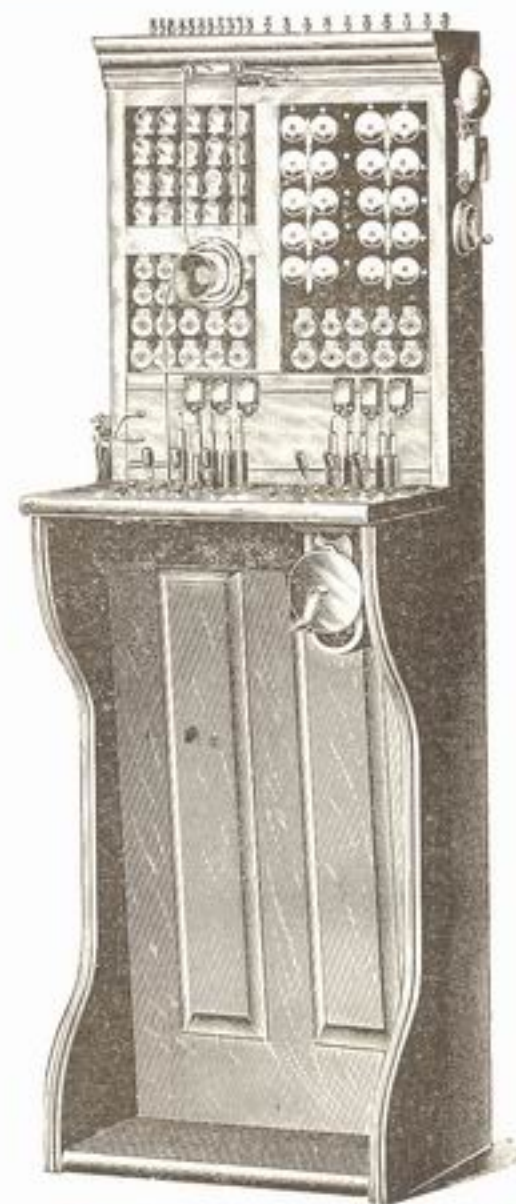
No. 2 SWITCH BOARD 20 Drops for Series Exchange Lines and 10 Gongs and Jacks for Bridge Lines
