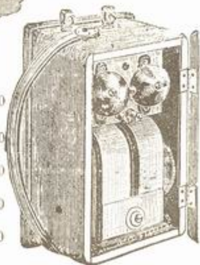
No. 4 SWITCHBOARD GENERATOR. For Series or Bridging Lines, 50,000 Ohms.
