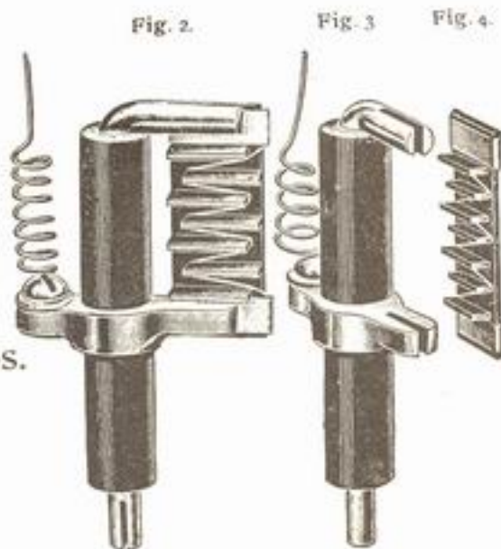
Fuses for Fused Cable Box.
