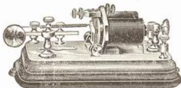
W. U. Standard Relay.
