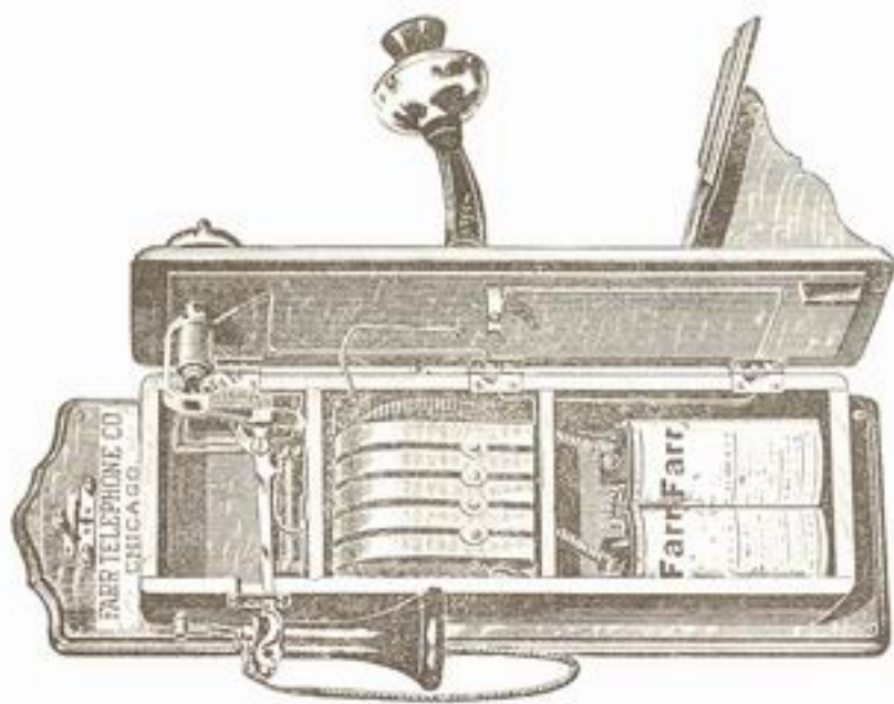
TELEPHONE NO. 14—OPENED.
