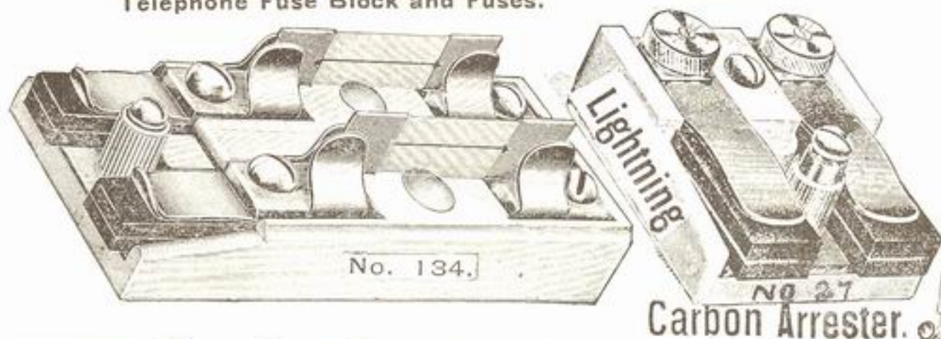
Telephone Fuse Block and Fuses.
