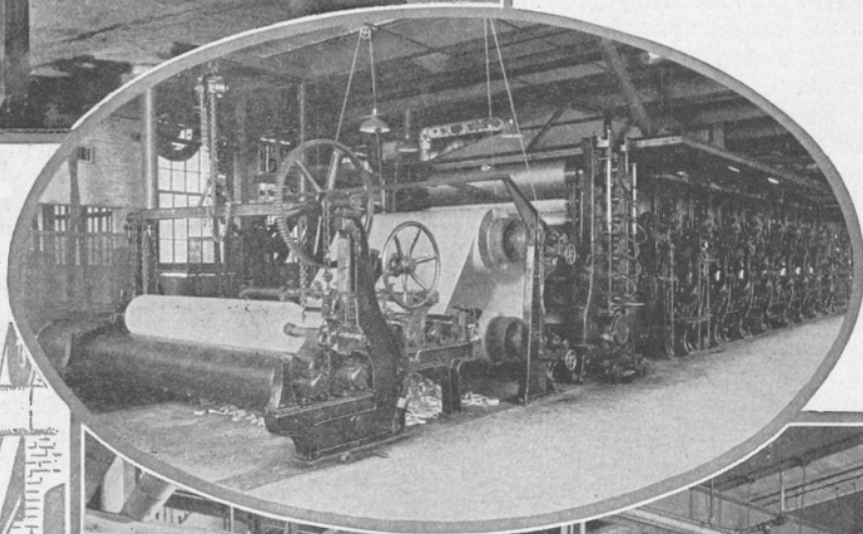
Below—The dry end of a paper making machine where paper is dried, calendered and rolled.
