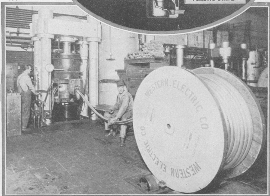
As the sheathed cable comes from the lead press it is wound on a reel which is turned slowly by the rollers under it.
