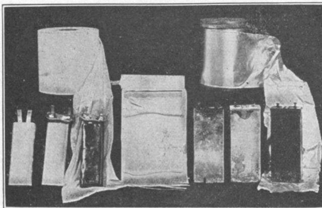
Antimony is used in the manufacture of condensers. At the top are rolls of insulating paper and the foil containing antimony, in the center a condenser unit slightly unrolled, while in the lower view are (left to right) a condenser unit after baking and impregnating; unit with outside terminals in place; unit after dipping; a condenser before cleaning and painting, and at the extreme right the finished product.
