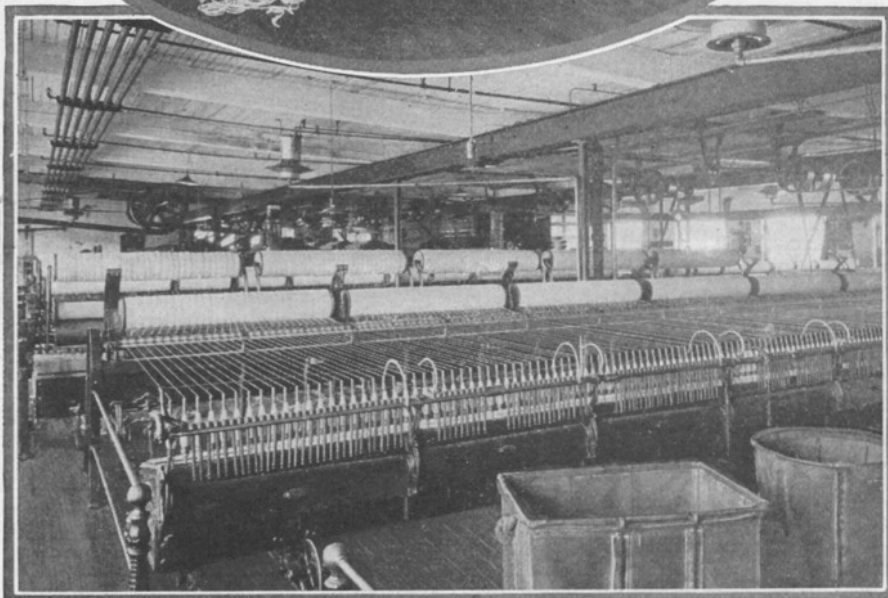
Spinning consists of transforming the roving into yarn by drawing and twisting, a process that includes winding the yarn on spools preparatory to weaving. The machine is called a spinning mule.
