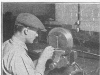
A die through which aluminum is forced by a press to form an I-beam.
