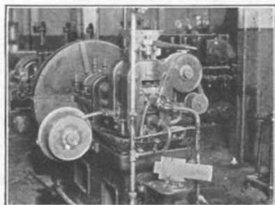
This rolling mill is used to make the thin strips of duralumin from which is made the diaphragm in the transmitter of your telephone.
