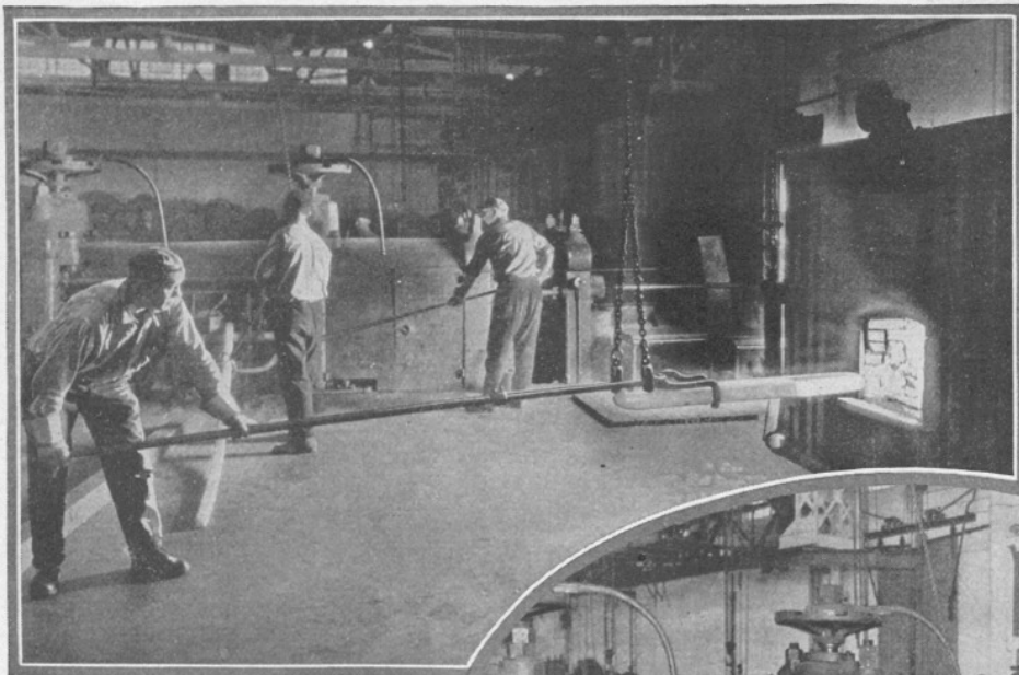
Taking a red hot bar of copper out of the furnace is the first step toward the rolls which turn the bar into a rod from which wire is drawn.
