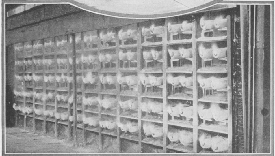
A zinc slab furnace where the zinc ore is reduced to molten zinc and, after tapping, cast into slabs.
