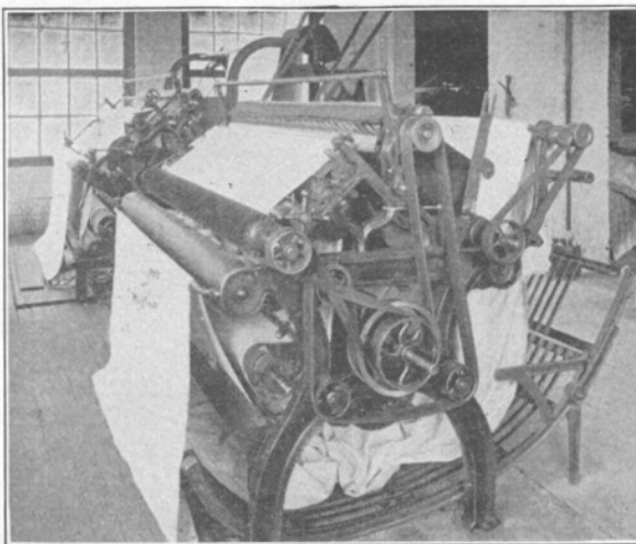
After the woven felt is made it is put through cleaning processes and dried and then sheared in a machine like the one above, which really gives it a haircut, trimming the fuzz off each side.
