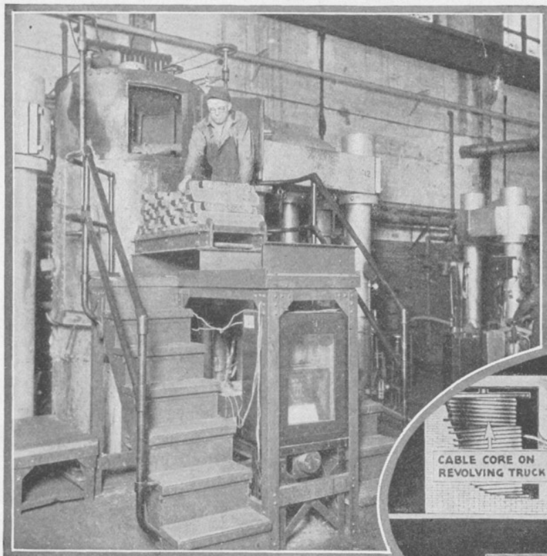
Left—Making lead sheathing to protect telephone wire starts with melting the pigs of lead for the lead press.
