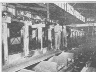
To get the grains of copper out of the ore by the flotation process the ore is crushed to a powder and then oil and water are mixed with it and air is forced through, forming a froth to which the copper grains adhere and from which they are skimmed off.
