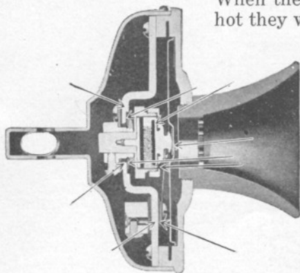
Mica is an insulator in about a dozen places in the transmitter of your telephone.
