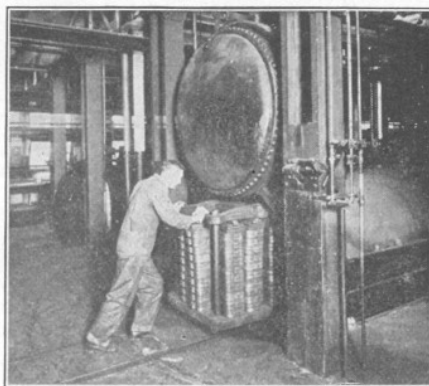
To bake and vulcanize the rubber for your telephone receiver, truckloads of moulds containing the rubber strips, shaped like half of a receiver, are pushed into an oven.
