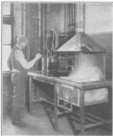
Carefully selected coal is used in the transmitter of your telephone. The operations of washing and drying granular carbon are performed with the simple machinery shown above.
