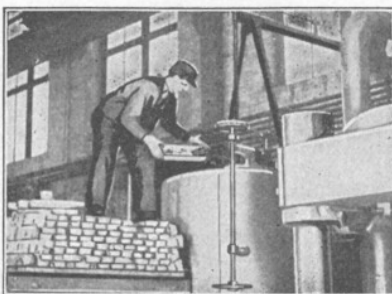
Pigs of antimony are melted with pigs of lead to form the alloy composing the sheaths of lead covered cables.
