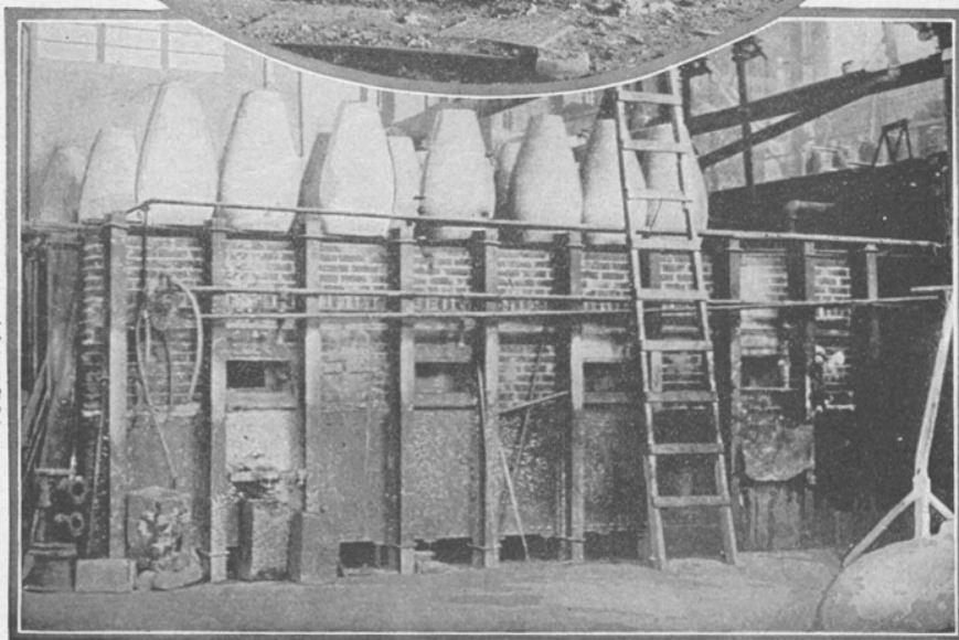
Refining furnaces separate the silver or zinc often found in the ore with lead.
