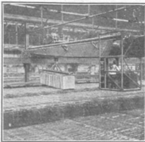
In the electrolytic process used to produce practically pure copper, the copper is made into anodes which are put into a solution and an electric current gradually deposits it on plates of pure copper. The copper plates or cathodes when built up by deposits are more than 99% pure copper.
