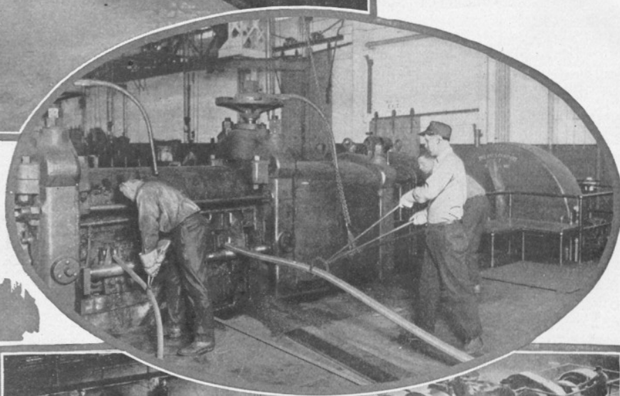
Taking a red hot bar of copper out of the furnace is the first step toward the rolls which turn the bar into a rod from which wire is drawn.
