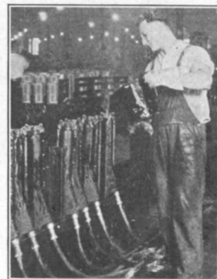
Asphalt in cable terminals, used when telephone wires are joined to a lead covered cable used as a main voice highway, prevents moisture working in among the wires and spoiling the insulation, thus enabling currents of electricity to stray from their proper paths.
