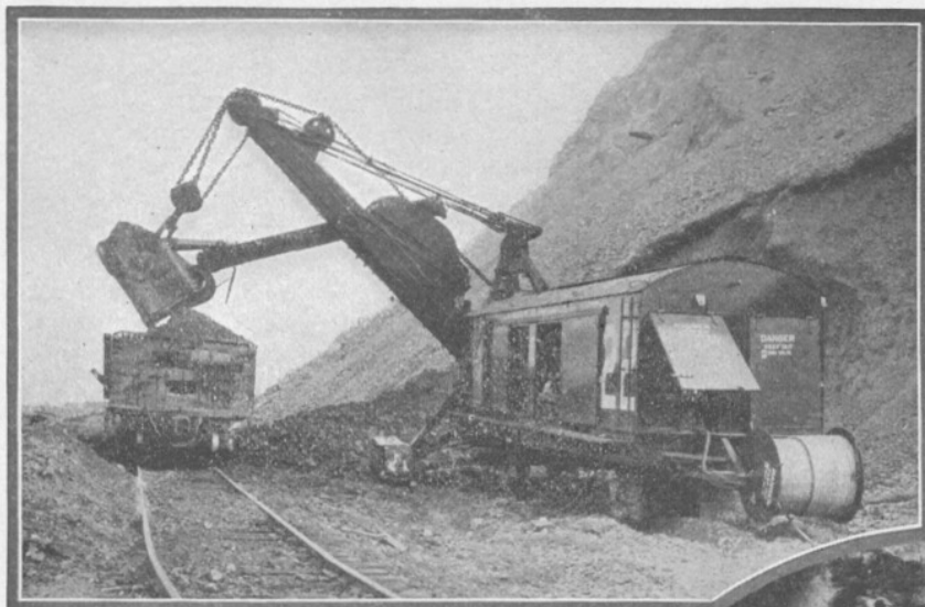
Copper ores in loose soil or from hillsides torn down by blasting are dug and loaded to send to the smelters by means of electric or steam shovels.
