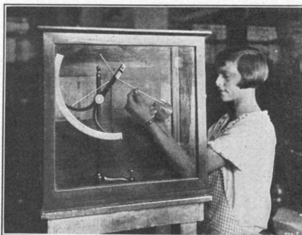
Inspecting aluminum foil to make sure that the thickness is right. Disks punched from each end of a strip of foil are one after the other attached to the arm of the balance. The disks are the same size and should weigh the same if they are the same thickness. Therefore, if the scale of the balance reads too much or too little the inspector knows the strips are not of even thickness.
