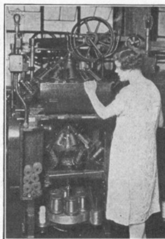
Silk and cotton are here being braided on telephone cords.
