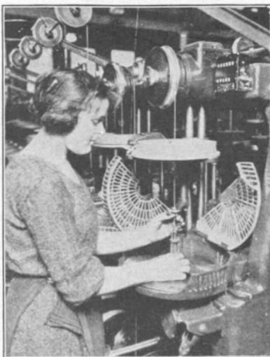
A strip of insulating paper is wrapped around each copper wire for lead covered cable. Different colors identify the wires. In the closeup the wire is seen coming up through the center of the flat roll of paper while the bobbin spins around it, wrapping the paper on in a long spiral.
