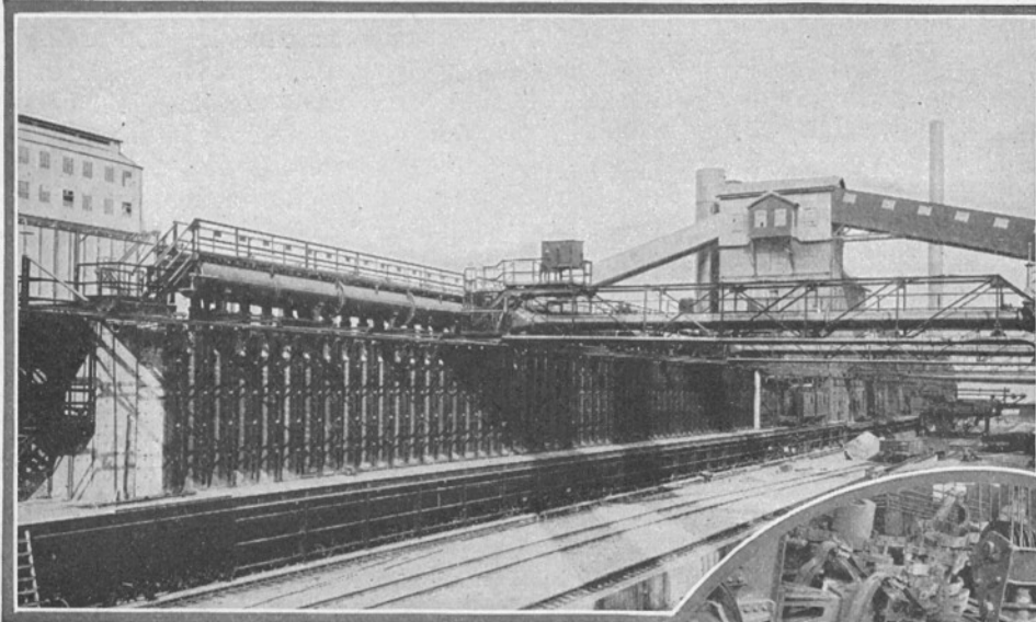
Part of the operation of iron and steel making is coke making. To make coke, coal of the kind needed is heated in ovens like these to get rid of the volatile materials (gases, etc.)
