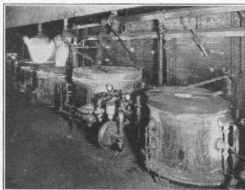
The granular carbon (coal) is roasted in ovens like these and it is in these operations that the gases leave the carbon in the flame shown coming from two of the ovens.
