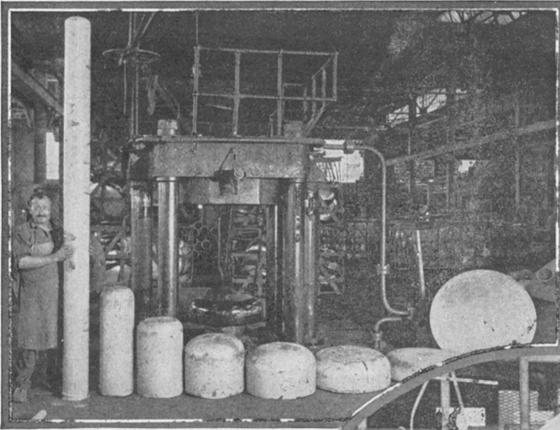
The flat disk of aluminum at the right changes shape, as shown from right to left, with each drawing process until it becomes the tubing at the extreme left.
