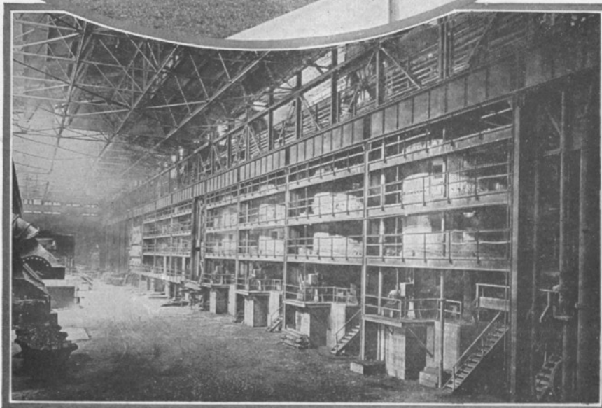
In zinc roasting furnaces the zinc and lead sulphides are converted into sulphate and oxide, the excess of sulphur is expelled and the iron and other metallic substances in the ore are oxidized to make a product suitable for leaching.
