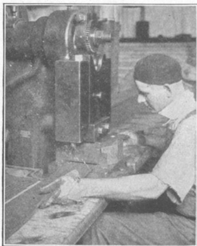
From long narrow strips of soft rubber, machines punch out pieces, shaped like half of the receiver rolled out flat.
