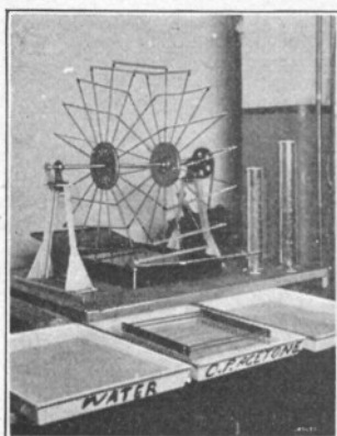
One after another thin strips of aluminum are immersed by this machine to learn how much, if at all, the aluminum is affected by corrosion from the bath they dip into.
