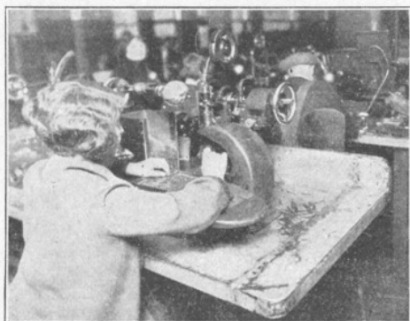
This girl is electrically welding contacts of gold, silver and platinum alloy on springs which will go into telephones.
