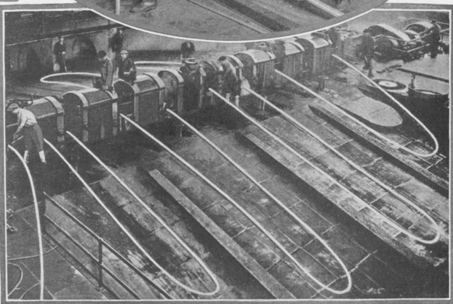
Each pass through the rolls reduces the thickness of the copper and increases the length, so that now the bar, which was originally 54 inches long and 4 inches square, has become 1200 feet long and only \frac{1}{4} inch thick.
