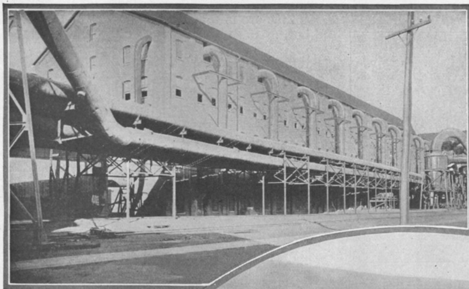
Left—Zinc oxide is sent through these big pipes by means of powerful blasts of air which blow the oxide to its destination.
