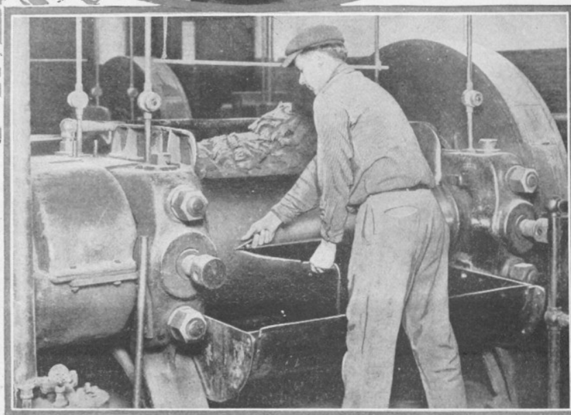
Partially rolled sheets are slit and put through the rollers again and again to knead in the sulphur and other ingredients for vulcanizing the rubber.
