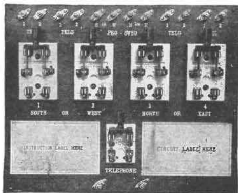
No. A-102142 Switching Panel
