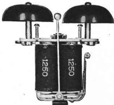
Ringer
