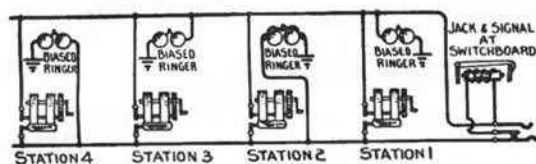
Pulsating Current 4 Party Selective Signaling—Magneto Systems
