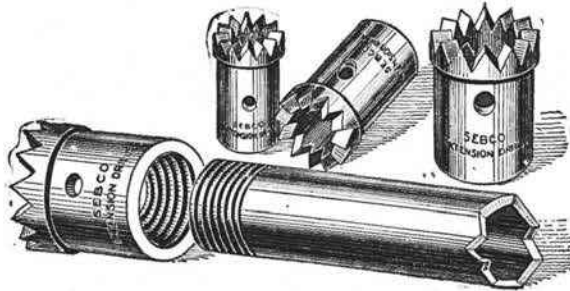
Extension Drills
