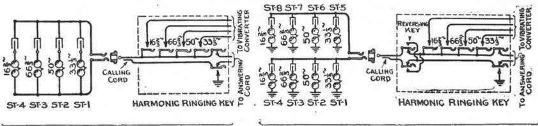
4 Party Selective 8 Party Selective Harmonic Selective Signaling—Magneto Systems
