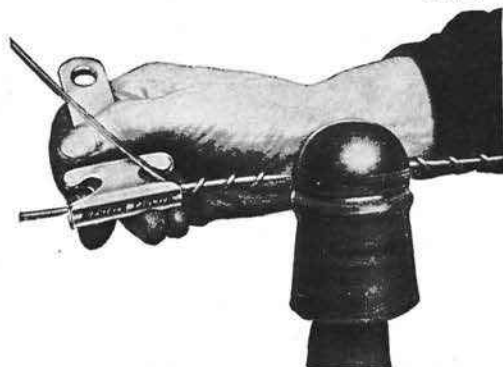
Method of "Tying In" with Tie Wrench
