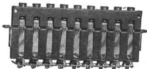
No. 69A Keys on No. 243 Mounting
