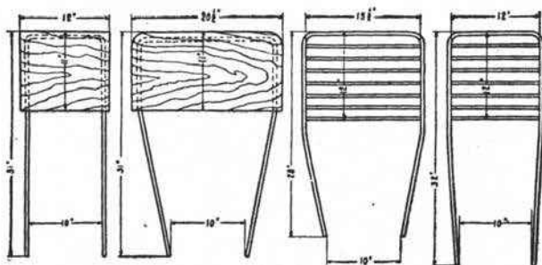
Pole Seats
