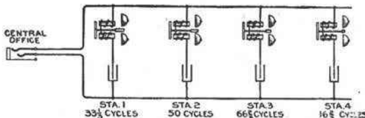
Harmonic Selective Signaling—Central Battery Systems 195
