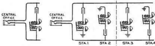
Individual Line 2 Party Selective 4 Party Semi-Selective Central Battery Systems
