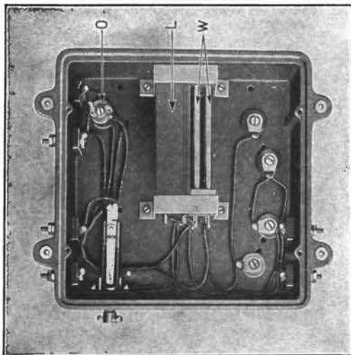
Bottom View of No. 84D Interrupter
