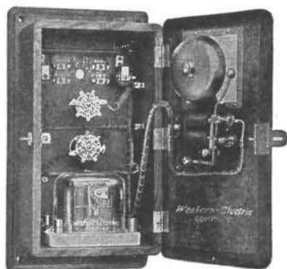
No. 101A Selector Set Open
