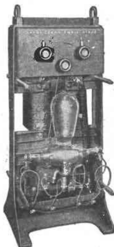
Type AT Rectifier Cover Off
