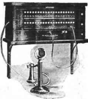
No. 1801 Switchboard Wall Type System A
