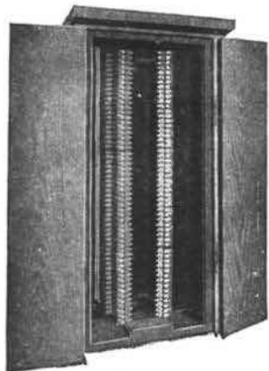
No. 17F Cable Terminal Open, with Protectors
