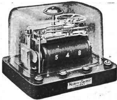
No. 60A Selector
