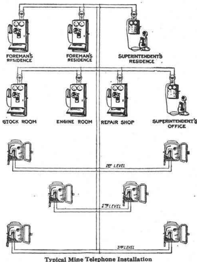
Typical Mine Telephone Installation
