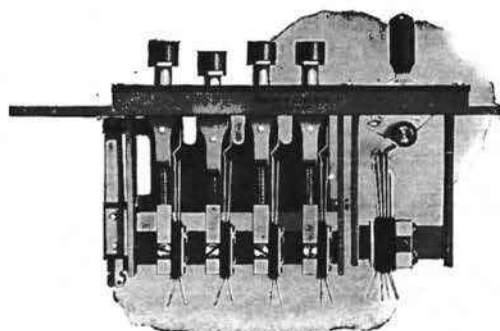
No. 468A Key
