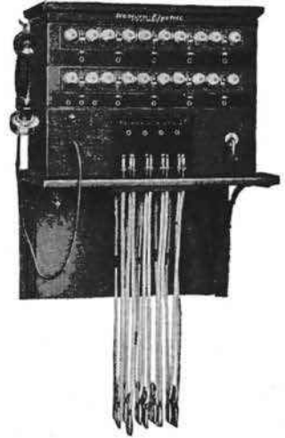
Wall Type—20 Lines Consists of: 1—AA-1 Top Unit 1—BA-7 Line Unit 1—BB-7 Line Unit 1—CA-1 Cord Unit 1—D-1 Supporting Unit
