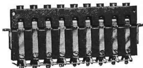
No. 243 Key Mounting Equipped With No. 69A Keys
