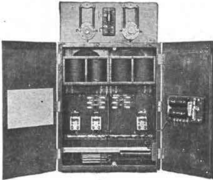
No. 53A Selector Apparatus Case
